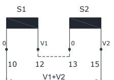
Serial connection double voltage
